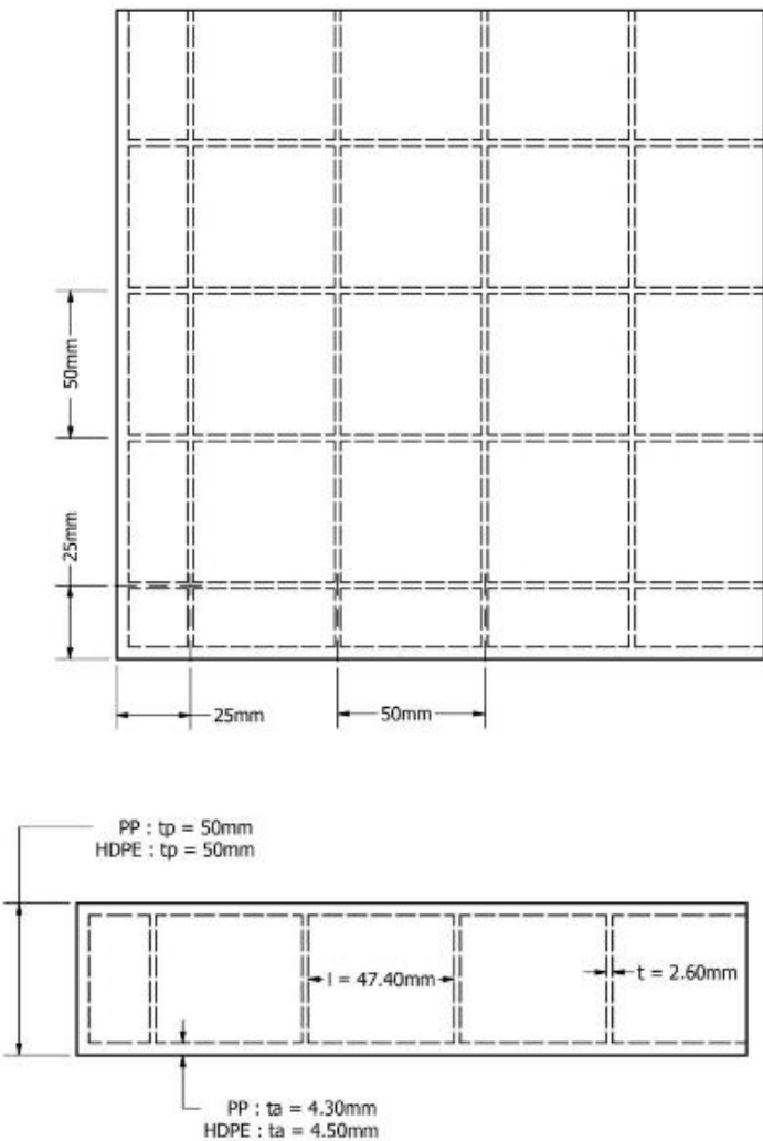
Figure 4.2 - Simplified technical drawing of a Multipower Panel 50/50
